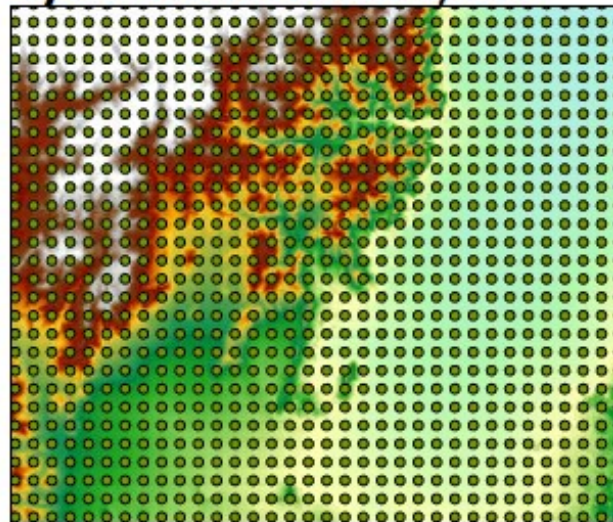
Systematic: Mean 1,615
