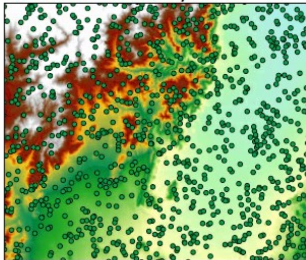
Random: Mean 1,600
