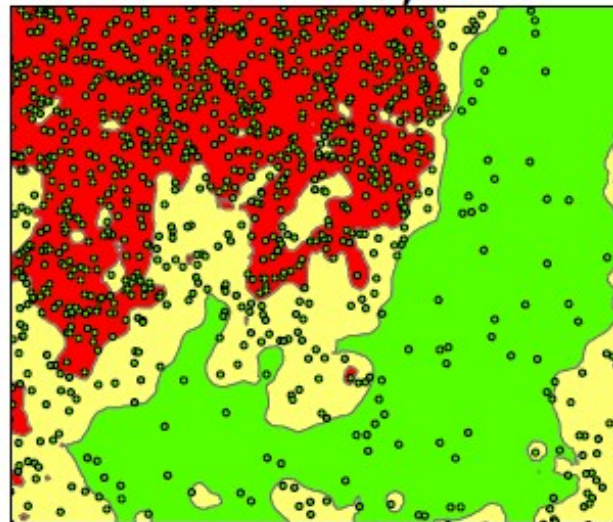
Stratified: Mean 1,838
