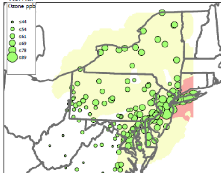
Kernal
