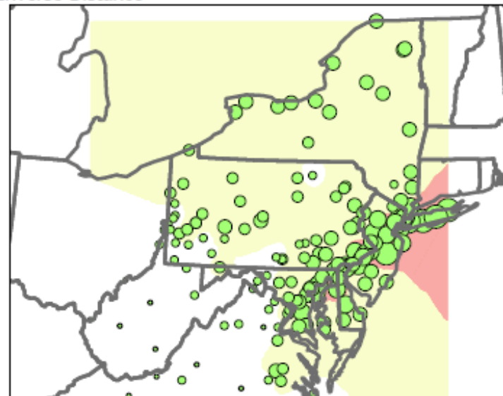
Inverse Distance
