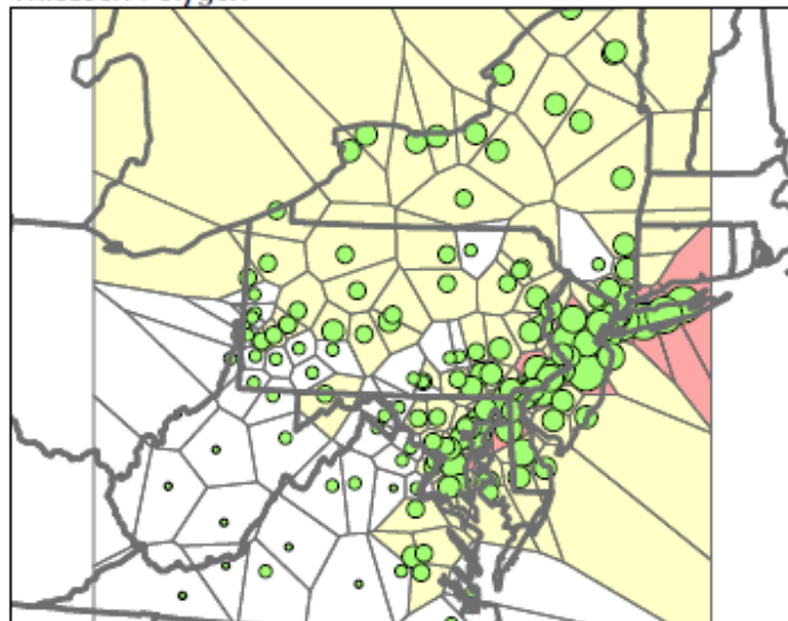
Thiessen Polygon
