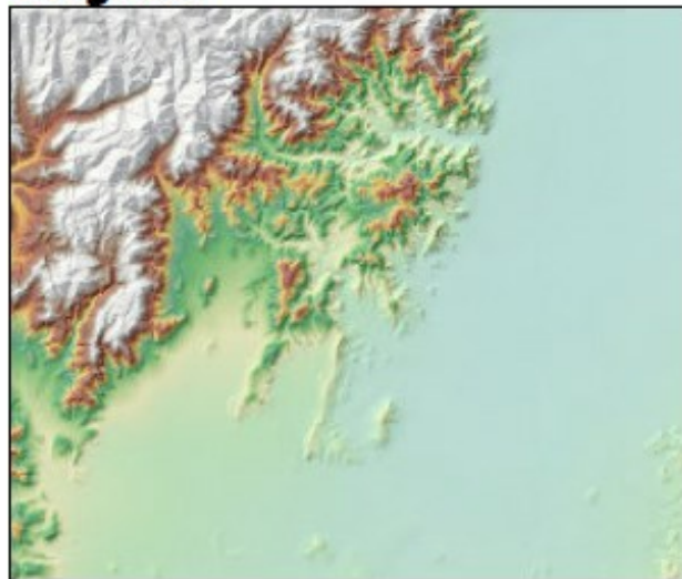
Original
